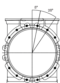
DN 450-DN 600
