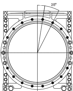
DN 700-DN 800
