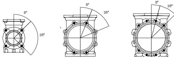
DN 50-DN 80
